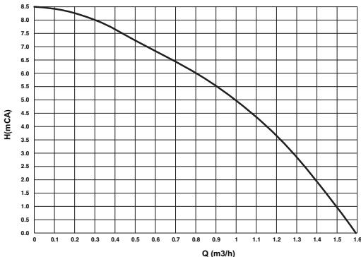
fig. 78- Residual head available for system
