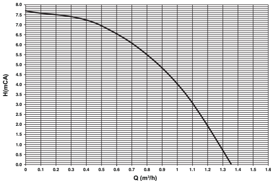
fig. 77- Residual head available for system
