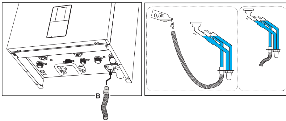
fig. 51- Condensate drain connection
