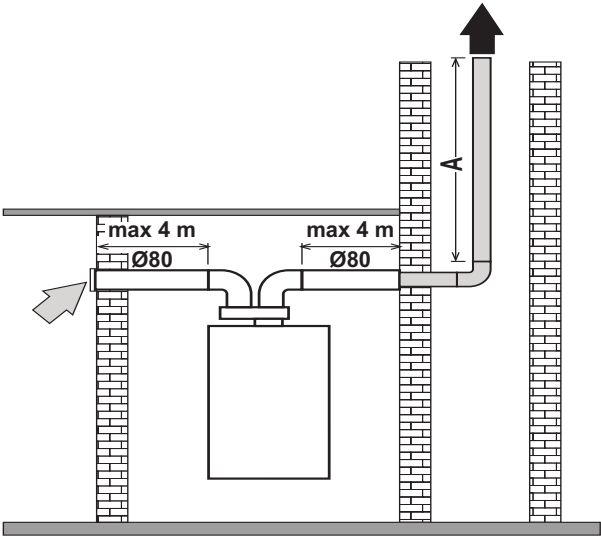
fig. 39- Layout for ducting only with flexible pipe
