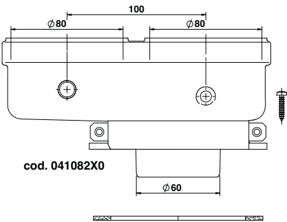
fig. 36- Starting accessory for separate ducts
