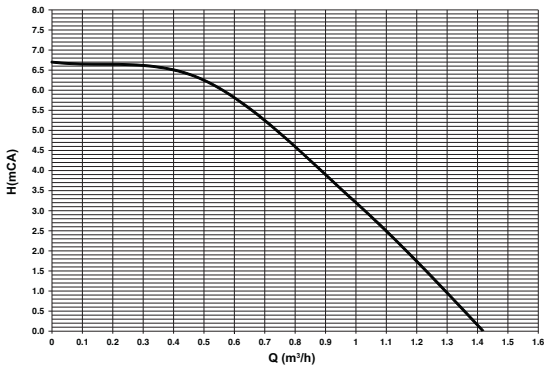
fig. 76- Residual head available for system
