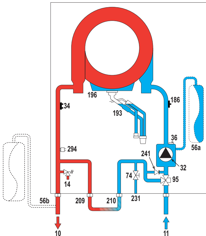
fig. 75- Hydraulic circuit
