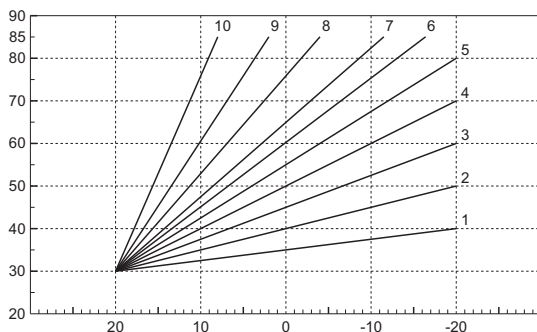
fig. 24- Compensation curves
