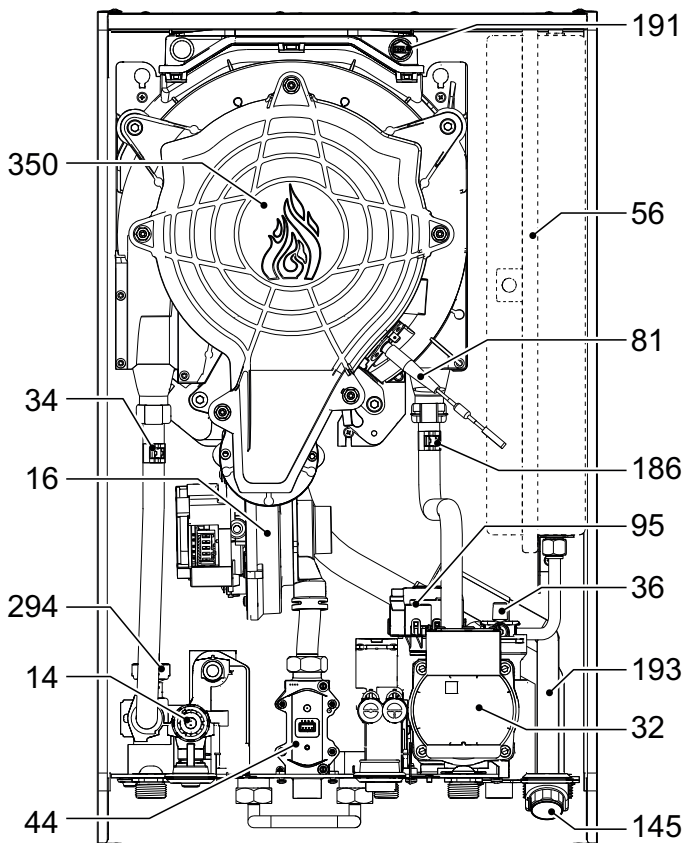
fig. 74- General view
