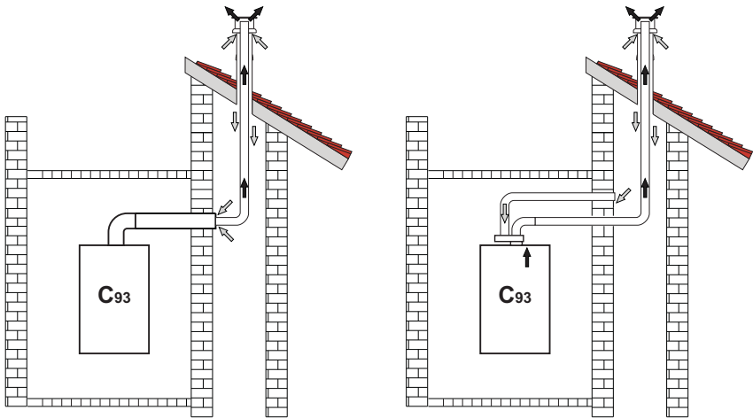
fig. 43- Examples of connection to collective flues (⇐ = Air / ➞ = Fumes)
