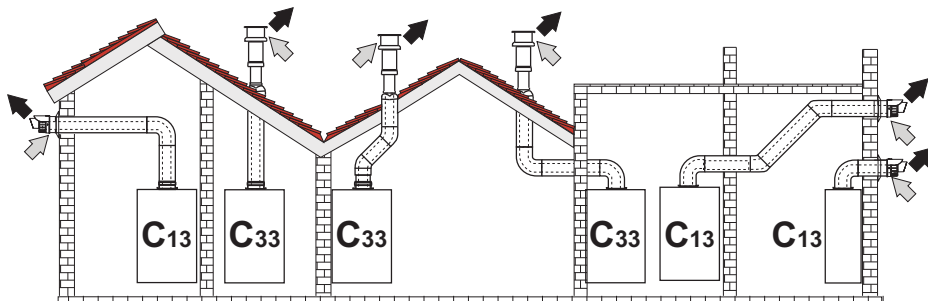
fig. 31- Examples of connection with coaxial pipes
